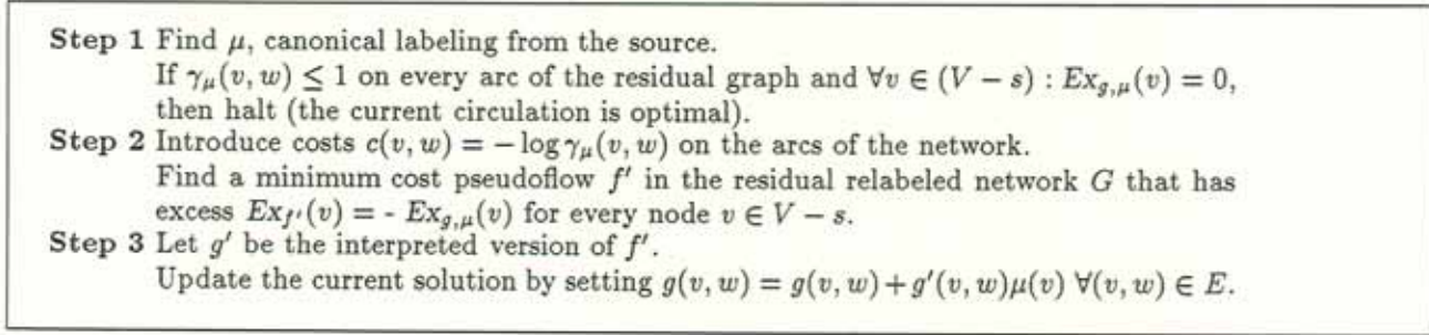
Figure 2: Inner loop of Algorithm MCF.
