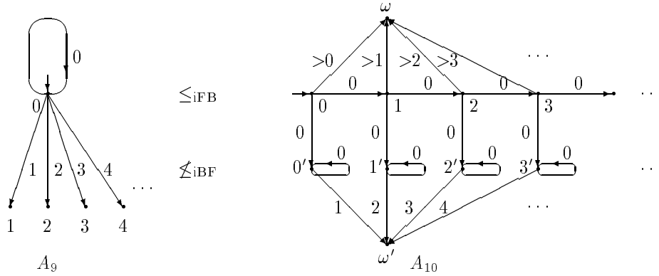
Figure 4: The difference between \leq_{\text{iFB}} and \leq_{\text{iBF}} .
